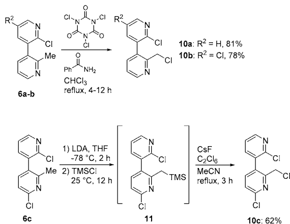
Scheme 3. Chlorination of the Picolyl Derivatives (6a–c)
